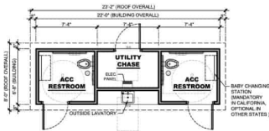
FLOOR PLAN
