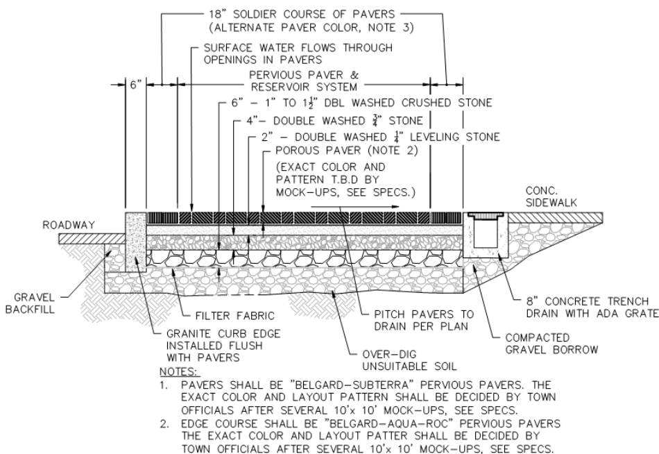
OPTION #1 – POROUS PAVER TYPICAL SECTION NOT TO SCALE
