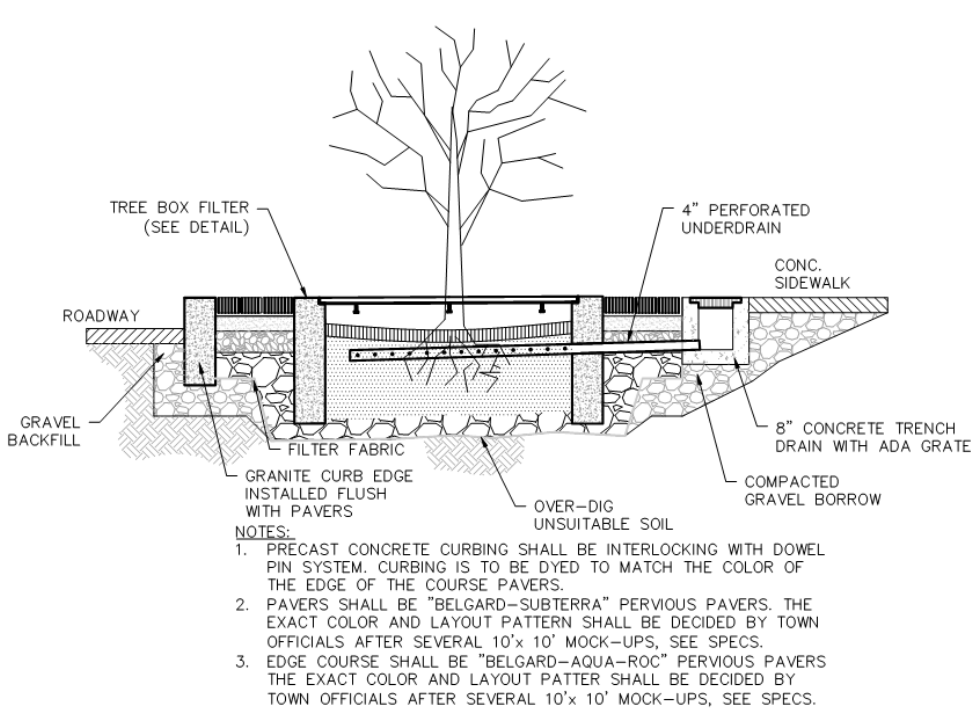
OPTION #2 – POROUS PAVER WITH TREE BOX SECTION NOT TO SCALE
