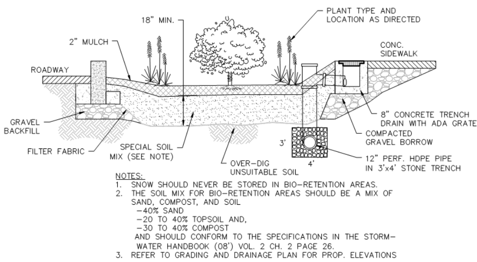
OPTION #3 – BIO-RETENTION AREA TYPICAL SECTION NOT TO SCALE
