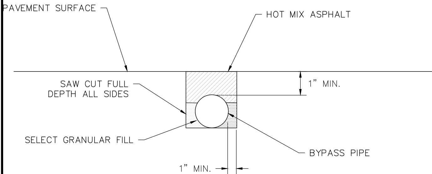
SIDEWALK AND STREET CROSSING
