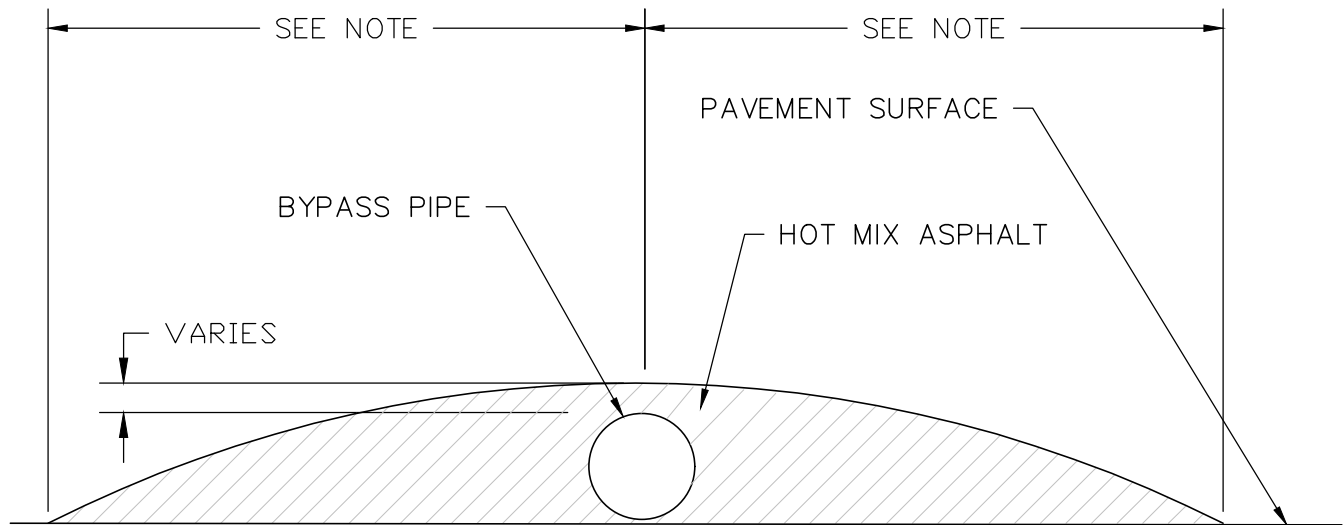
DRIVEWAY CROSSING
