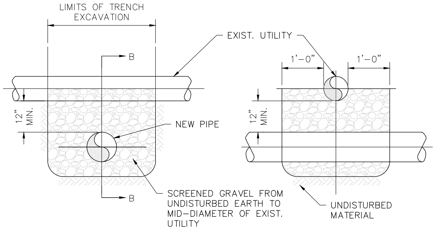
TYPICAL SECTION
