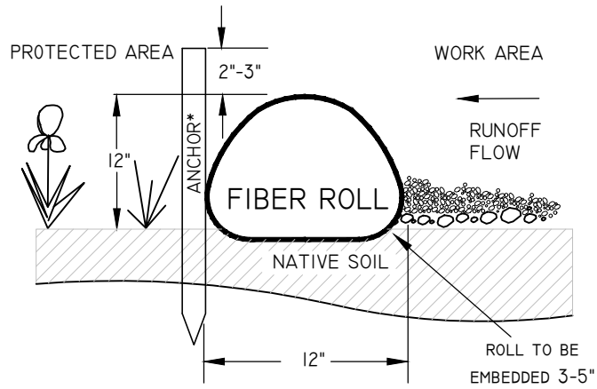
FIBER ROLL SECTION VIEW
