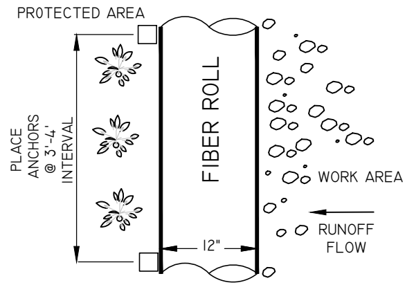
FIBER ROLL TOP VIEW
