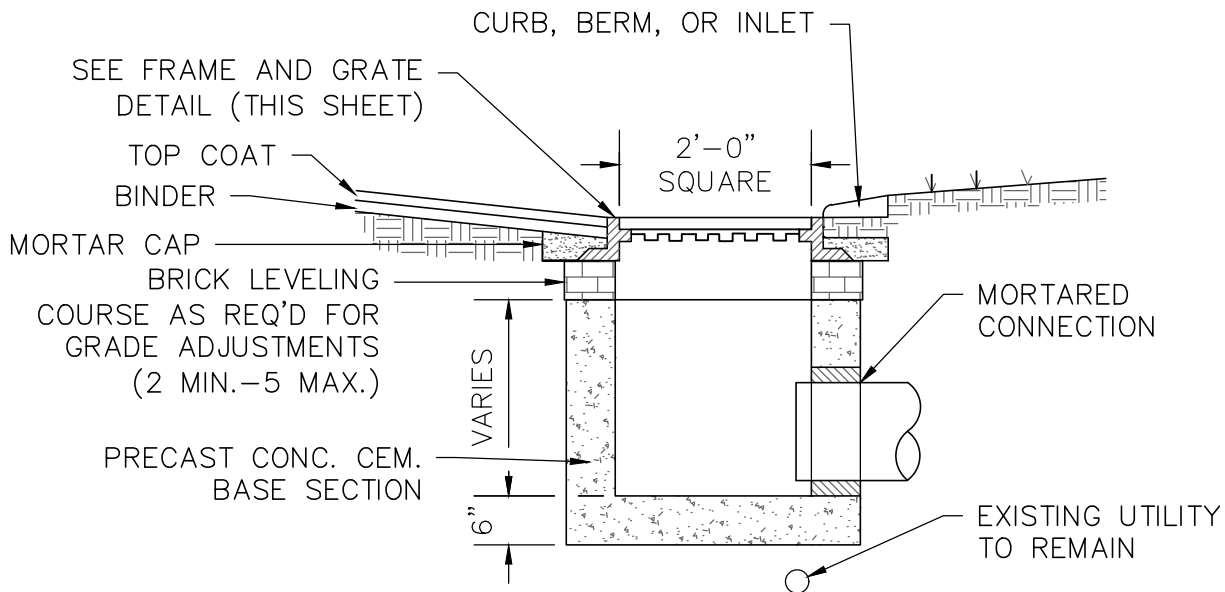
SECTION VIEW
